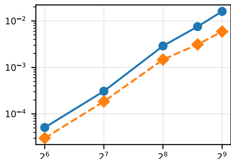
ill_conditioned, BLAS=8
