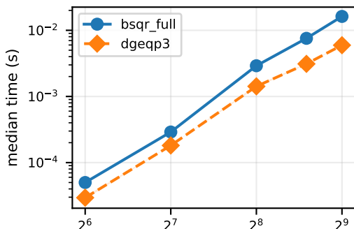
ill_conditioned, BLAS=1
