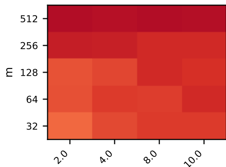
ill_conditioned, BLAS=1
