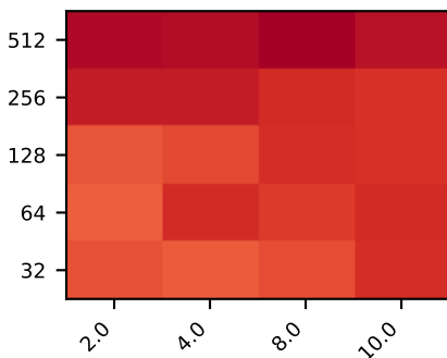
ill_conditioned, BLAS=8
