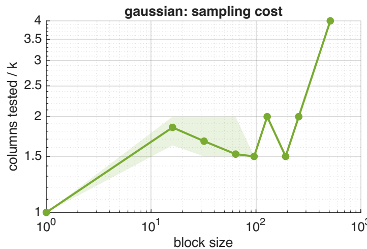
Effect of block size (running_mean threshold, k=128, n=8000)
