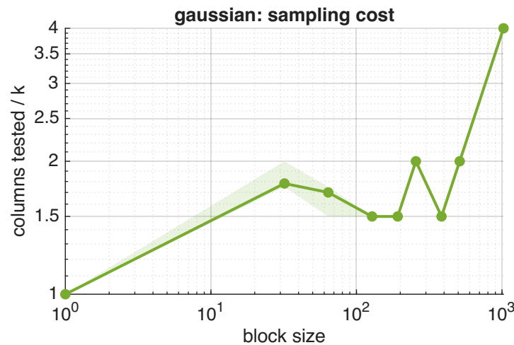
Effect of block size (running_mean threshold, k=256, n=8000)
