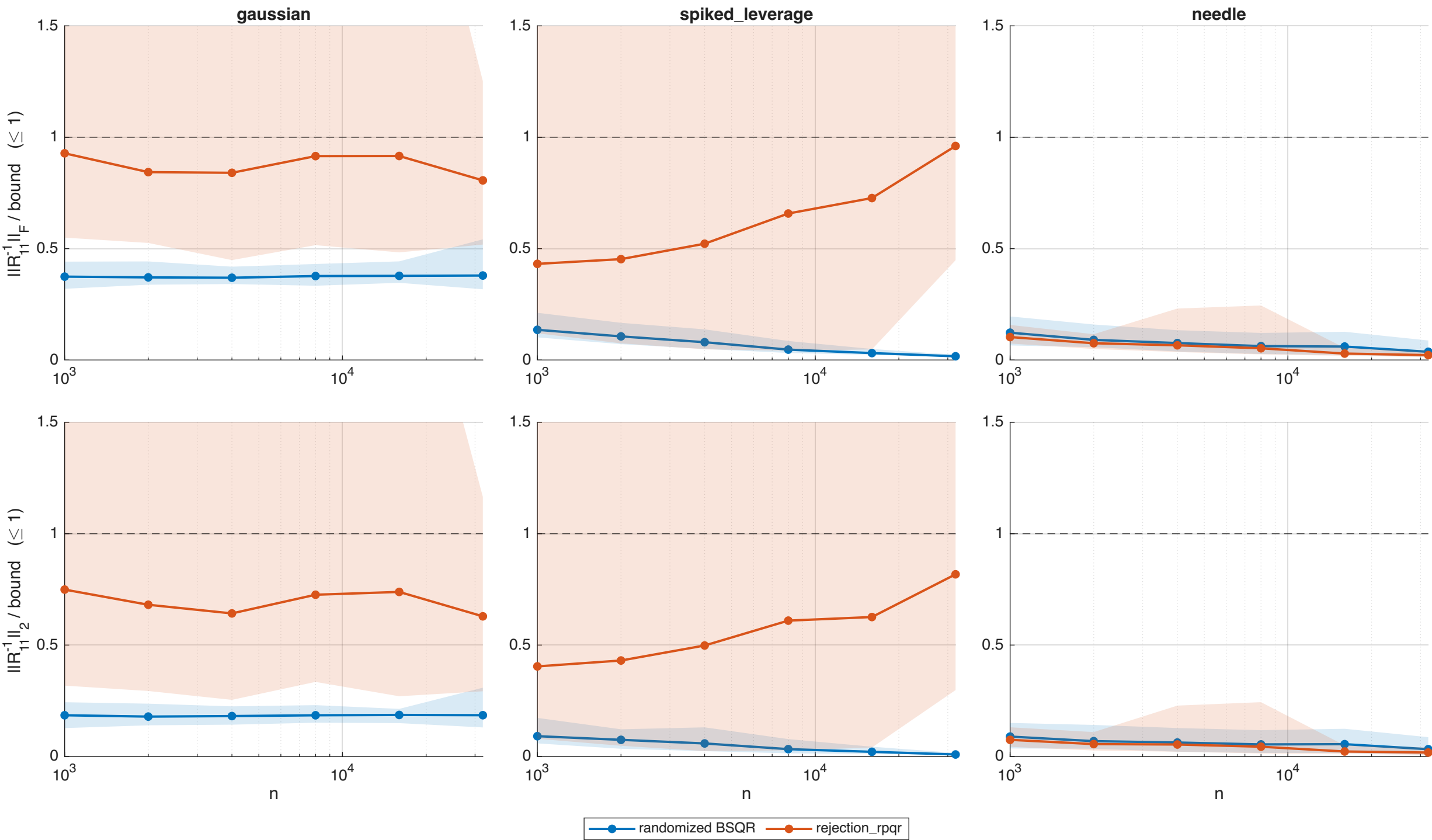
Selection quality vs the bounds (k=64, lower = better): Frobenius \|R_{11}^{-1}\|_F (top), spectral \|R_{11}^{-1}\|_2 (bottom)
