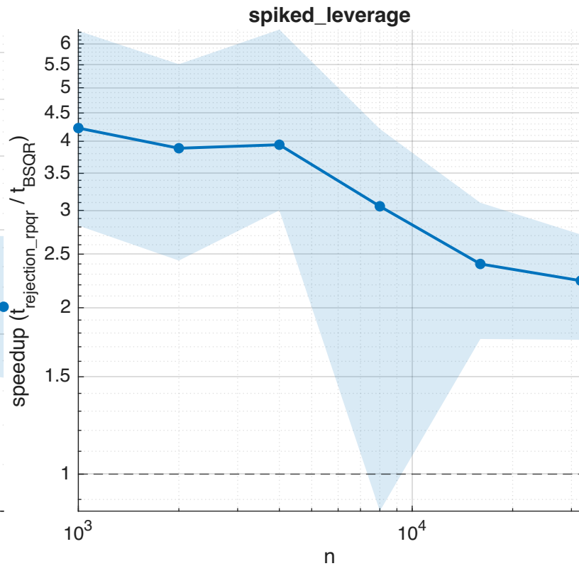
Speedup of randomized BSQR over rejection_rpqr ( t_{\text{rpqr}}/t_{\text{BSQR}} ) ( k=128 )
