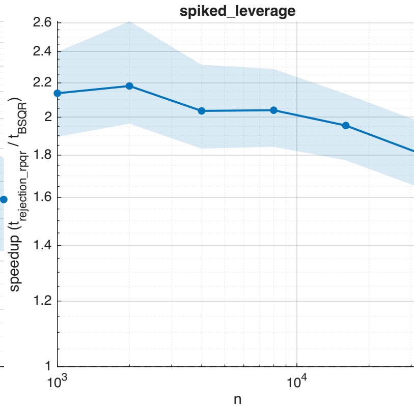
Speedup of randomized BSQR over rejection_rpqqr ( t_{\text{rpqr}}/t_{\text{BSQR}} ) (k=256)
