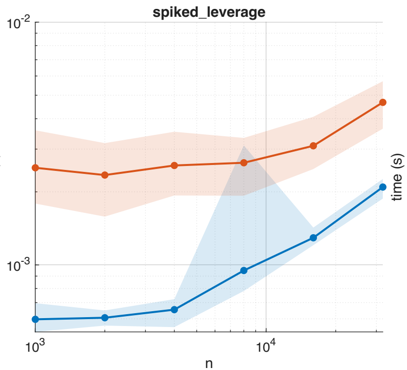
Runtime vs n (k=128)
