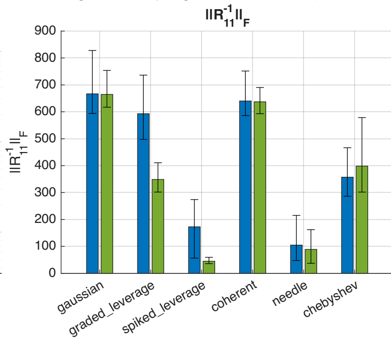
Uniform vs norm-weighted sampling across families (k=128, n=32000, block=128)
