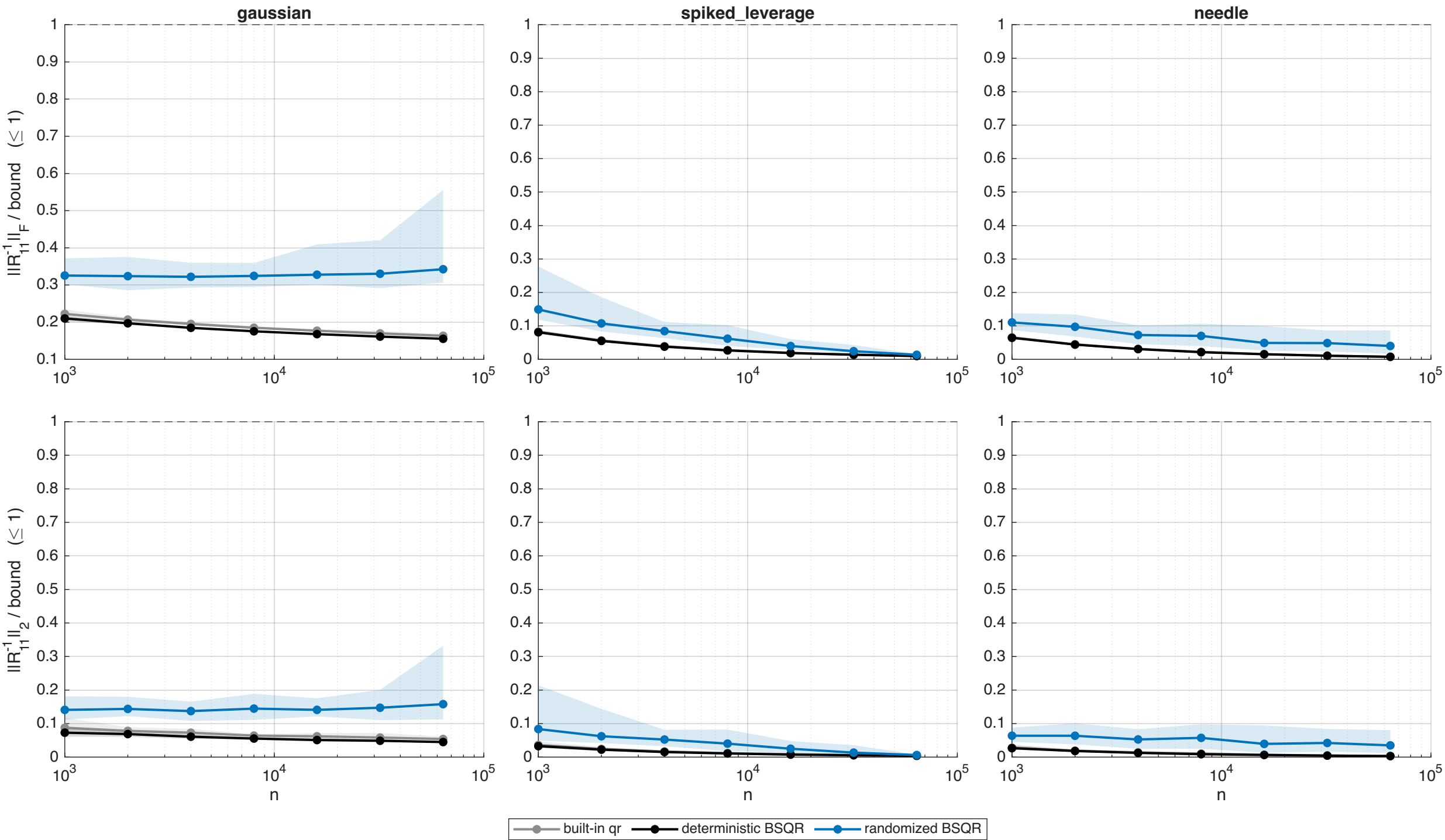
Selection quality vs the bounds (k=128, lower = better): Frobenius \|R_{11}^{-1}\|_F (top), spectral \|R_{11}^{-1}\|_2 (bottom)
