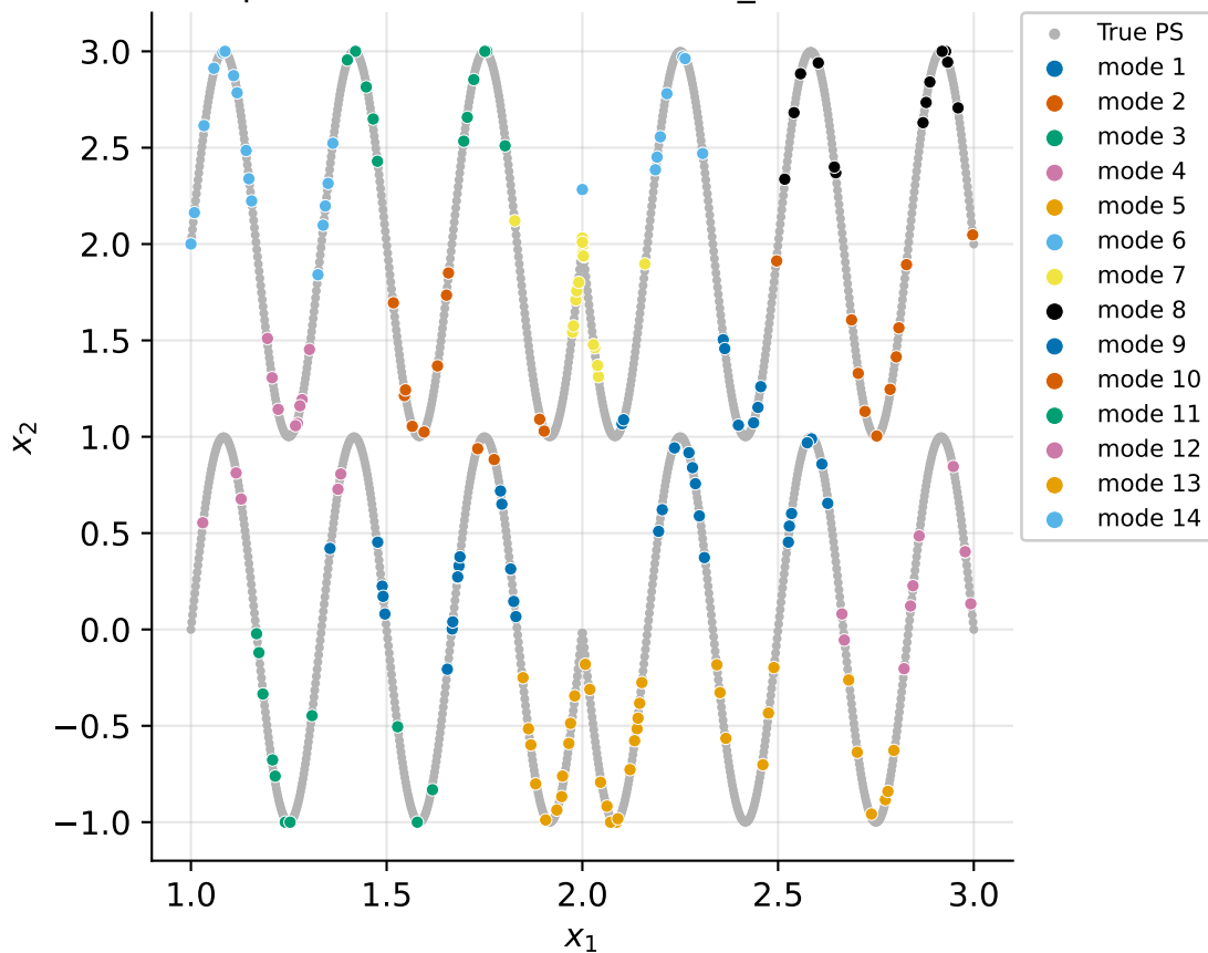
Decision-space modes -- MMF5 / EARS_MMOEA (14 modes)
