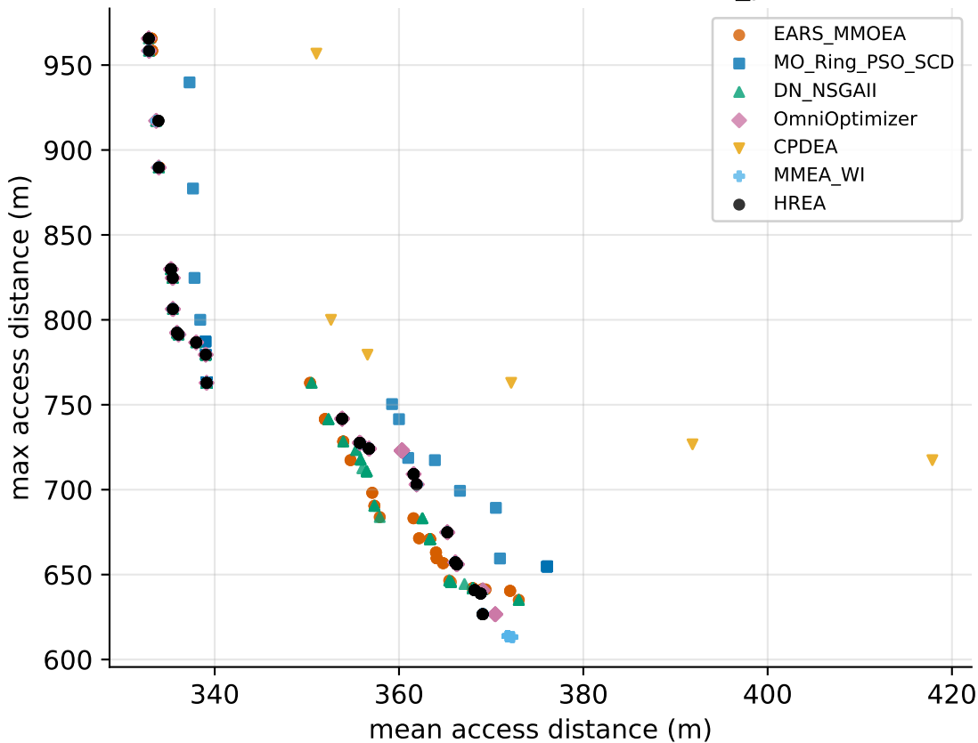
Placement Pareto front -- Macau_p11
