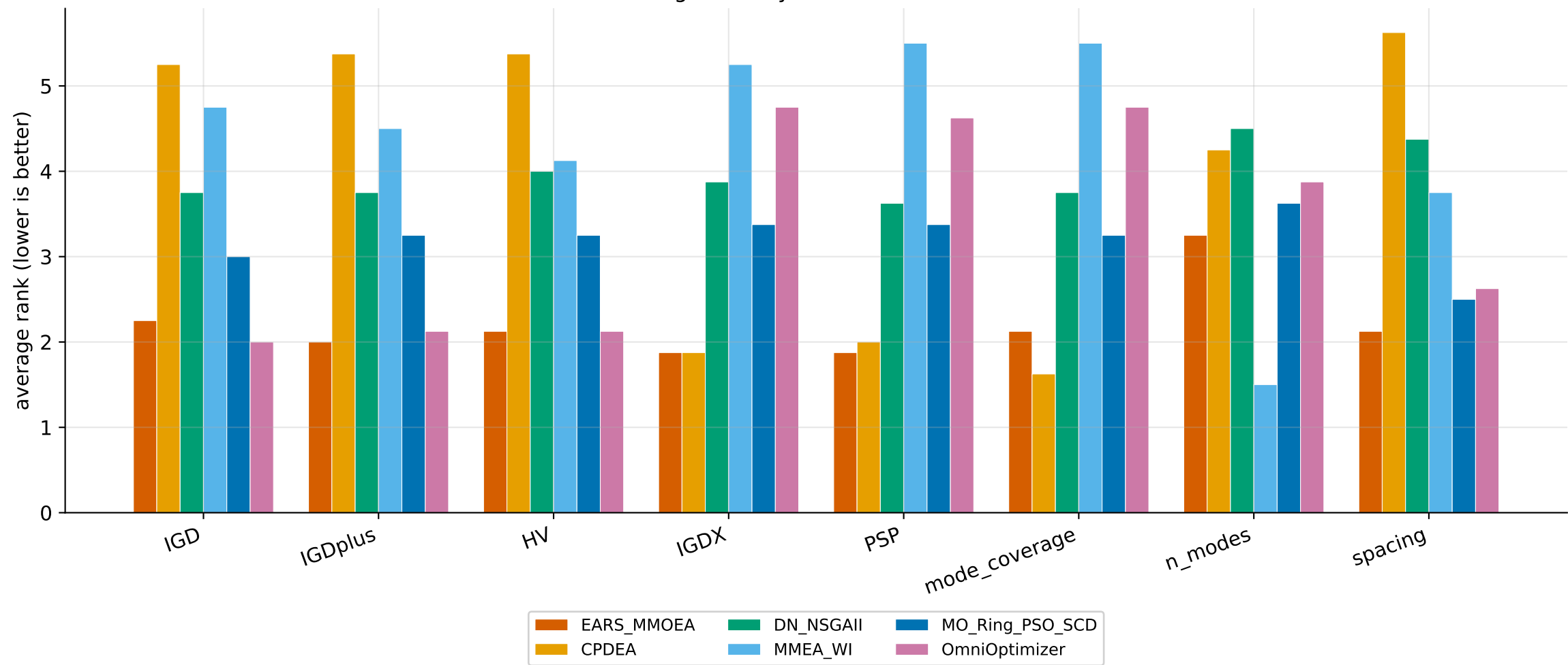
Average rank by metric -- benchmark
