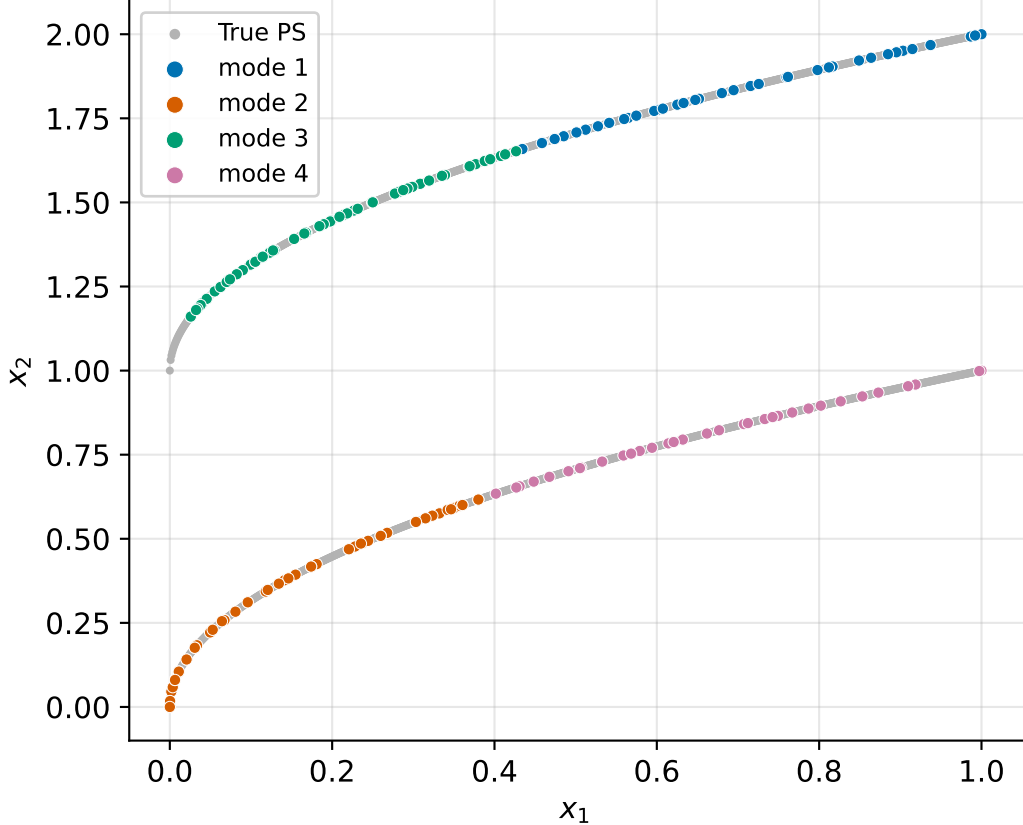
Decision-space modes -- MMF2 / EARS_MMOEA (4 modes)
