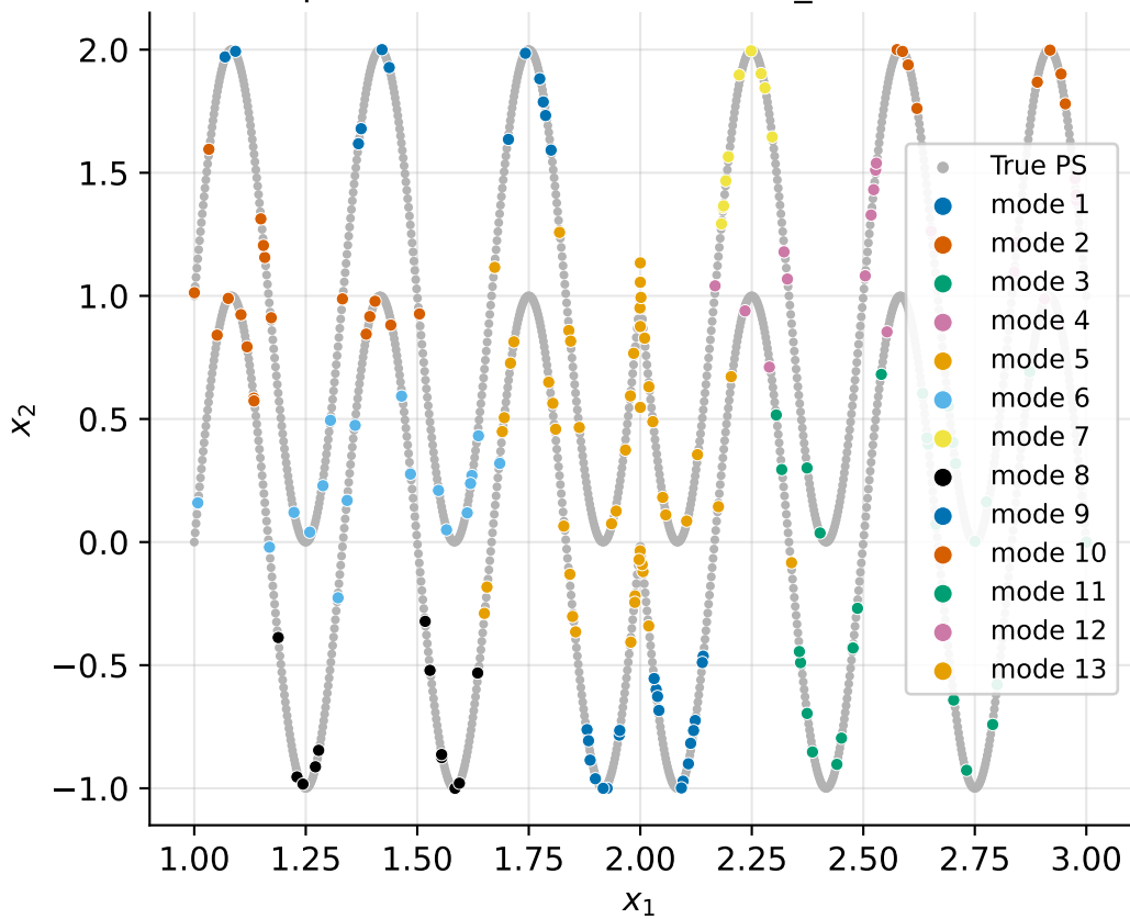
Decision-space modes -- MMF6 / EARS_MMOEA (13 modes)
