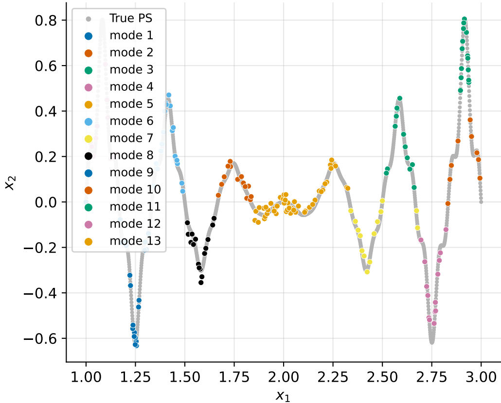
Decision-space modes -- MMF7 / EARS_MMOEA (13 modes)
