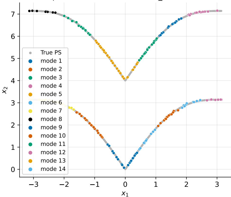
Decision-space modes -- MMF8 / EARS_MMOEA (14 modes)
