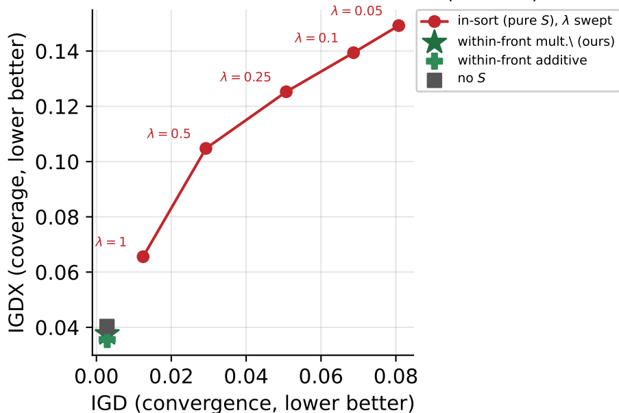
Placement: within-front dominates the in-sort curve (MMF1--8)
