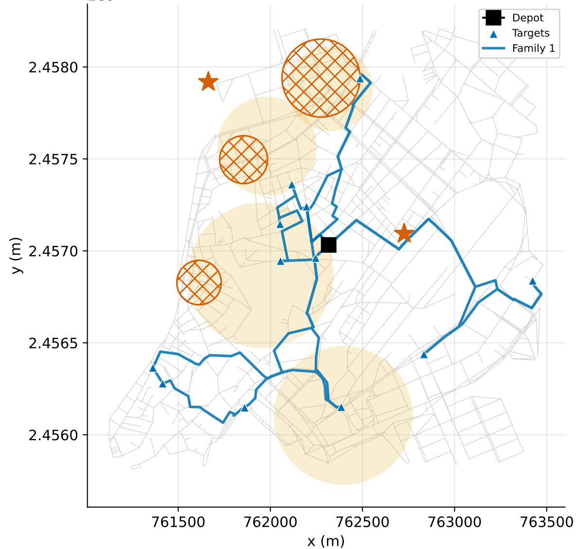
1e6 Pareto-equivalent UAV route families — Macau (s1)
