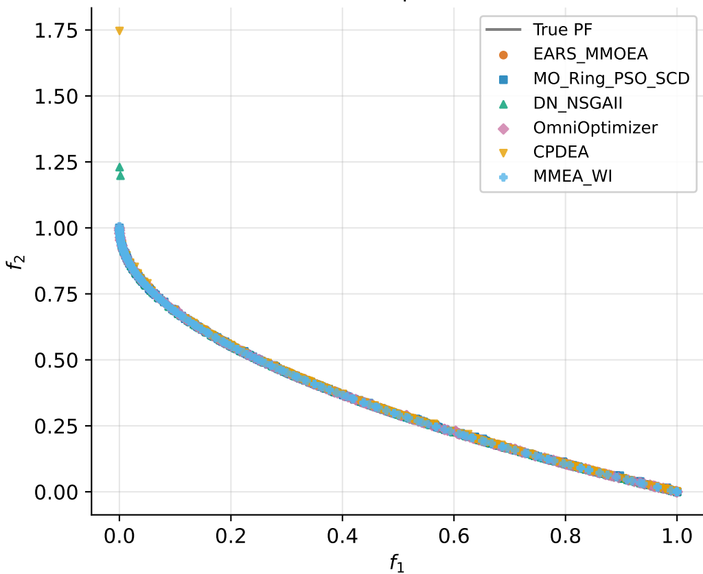
Pareto front comparison -- MMF1
