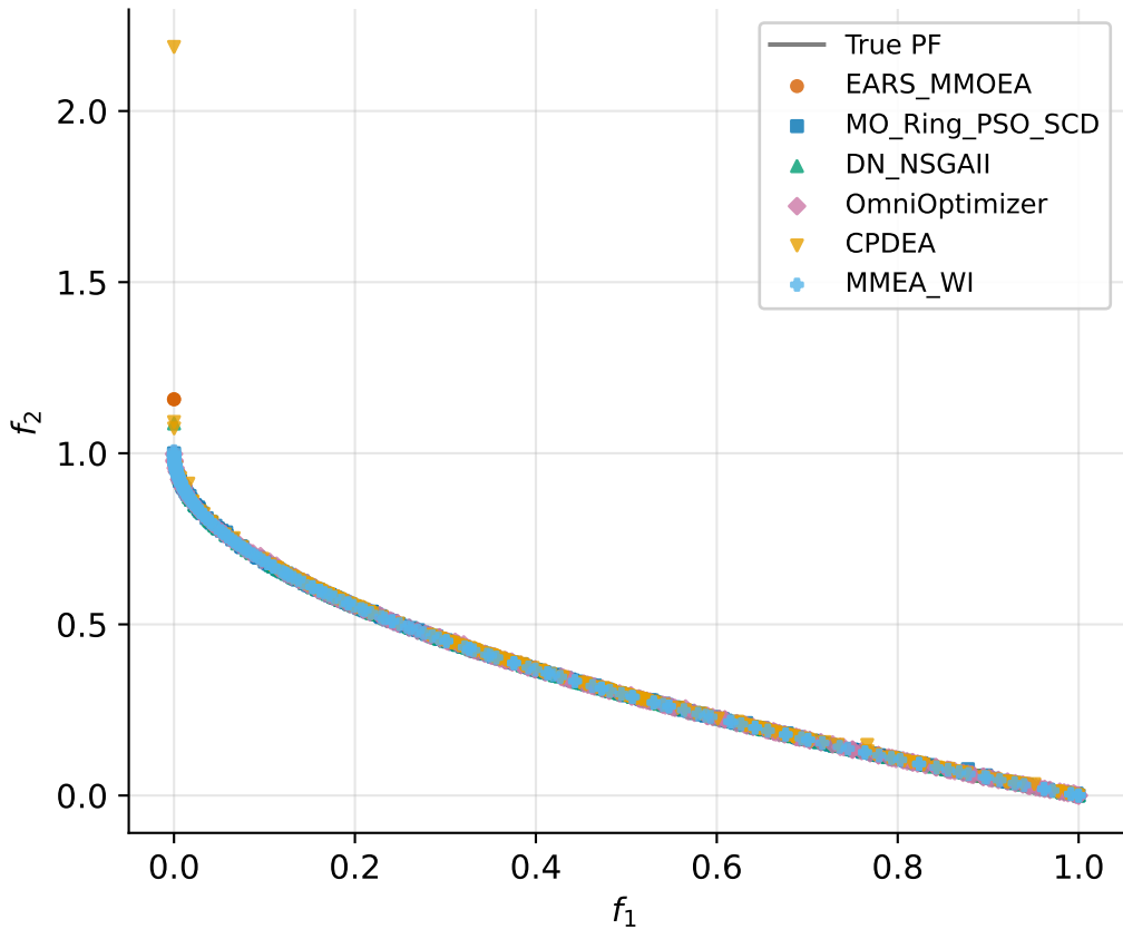
Pareto front comparison -- MMF5
