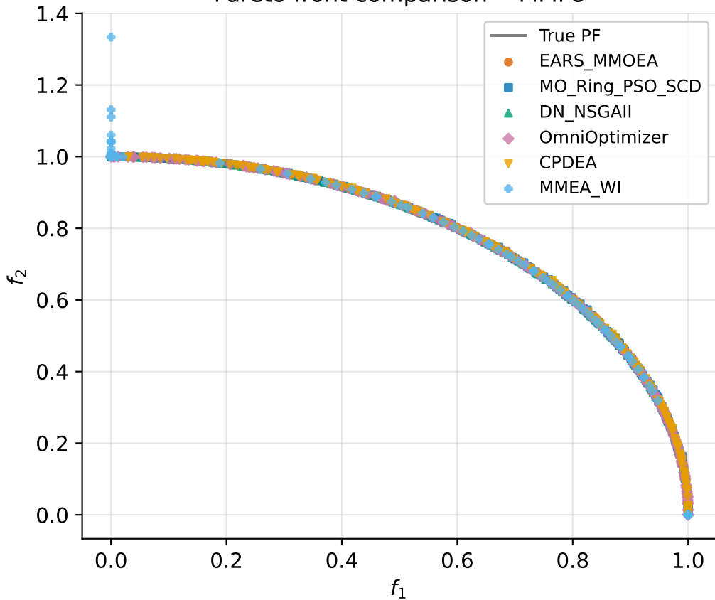
Pareto front comparison -- MMF8
