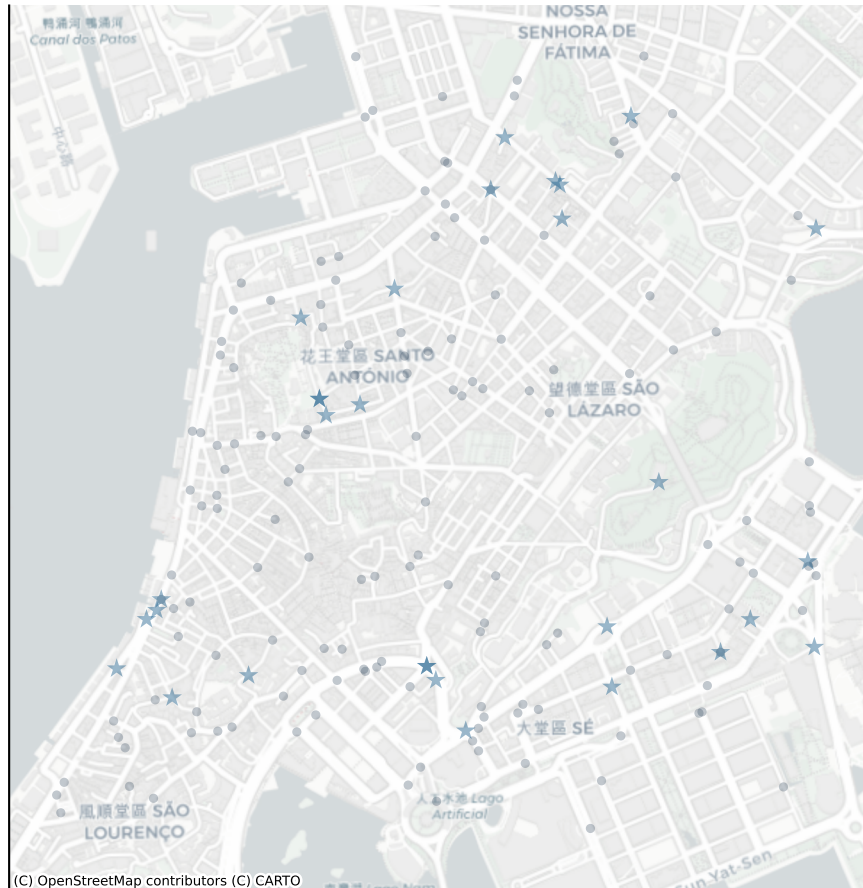
CPDEA mean 2.0 near-optimal layout modes (over 90 runs)
