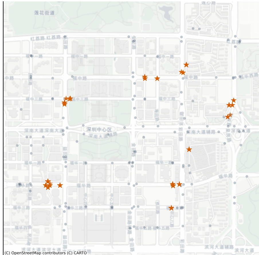
EARS_MMOEA (ours) mean 14.2 near-optimal layout modes (over 30 runs)
