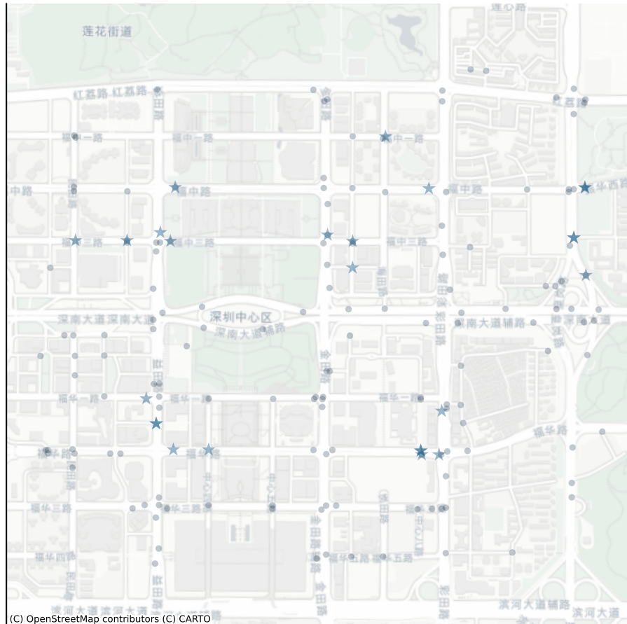
CPDEA mean 2.4 near-optimal layout modes (over 30 runs)
