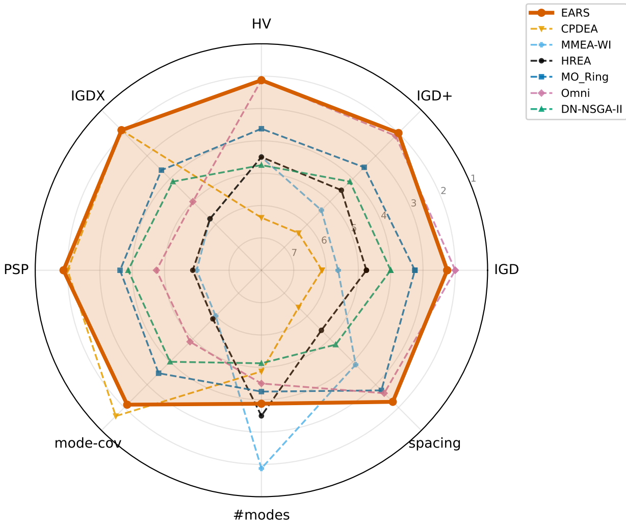
Benchmark average rank per metric (outer = best)
