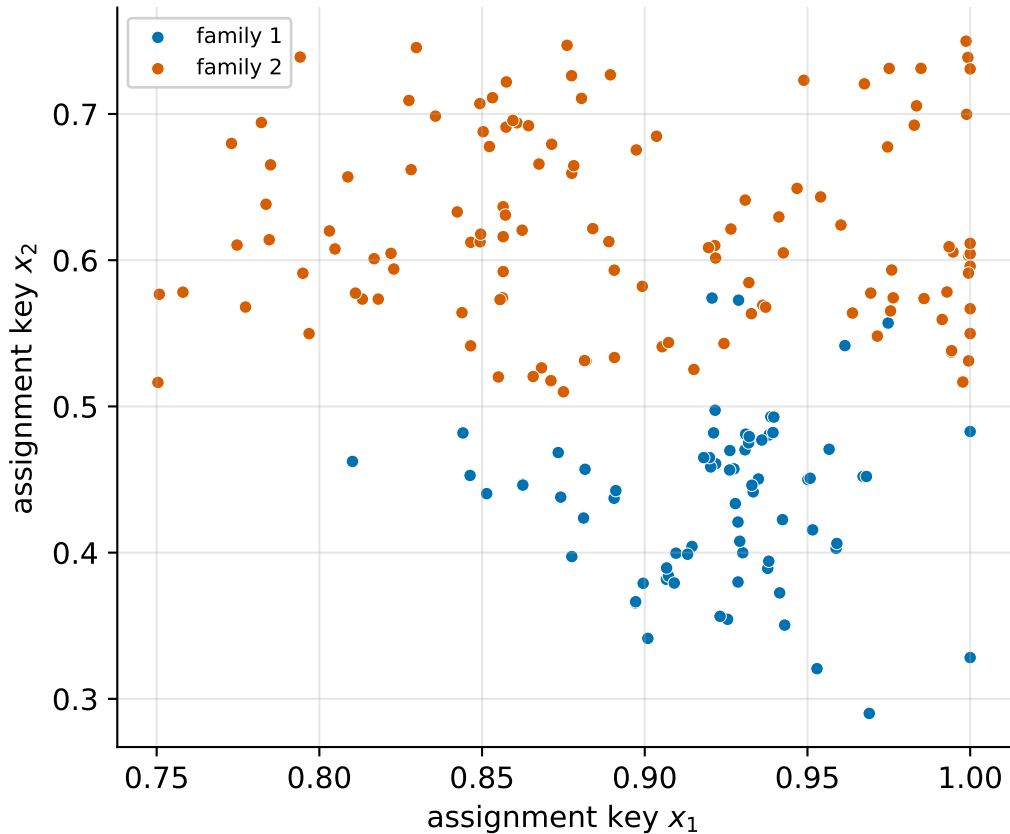
Decision-space route families — Macau_s1 (2 modes)
