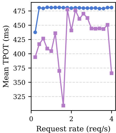
(c) Time per Output Token
