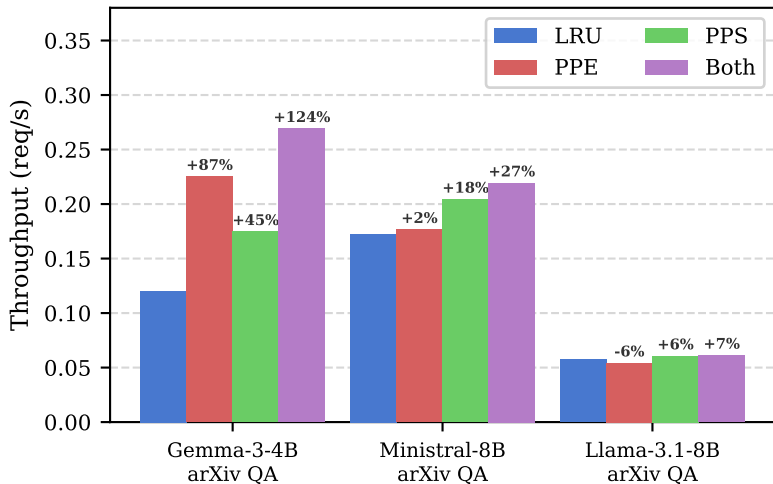
(a) Shared-prefix workloads
