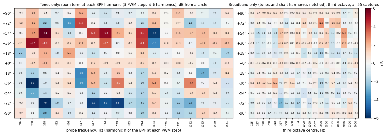
Fig. 2 · Left: the tone position term at each of the 18 probe frequencies (3 speeds \times 6 harmonics; prop7 and PWM 1200 excluded). Right: the broadband position term, tones and shaft harmonics notched, third-octave, all 55 usable captures at all speeds. Same colour scale. The left panel is the one-pager's problem; the right panel is the room for a broadband source.
