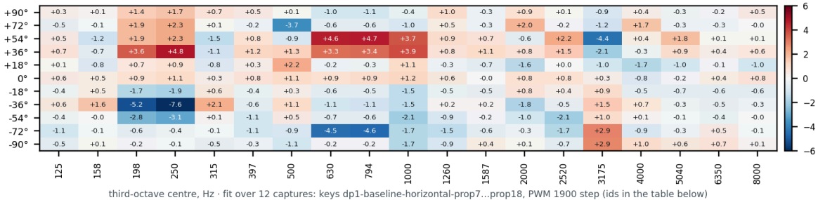
Fig. 3 · Two positions, twelve runs, three microphones
