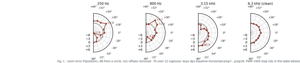
Fig. 1 · room error P(position), dB from a circle, mic offsets removed · fit over 12 captures: keys dp1-baseline-horizontal-prop7...prop18, PWM 1900 step (ids in the table below)
