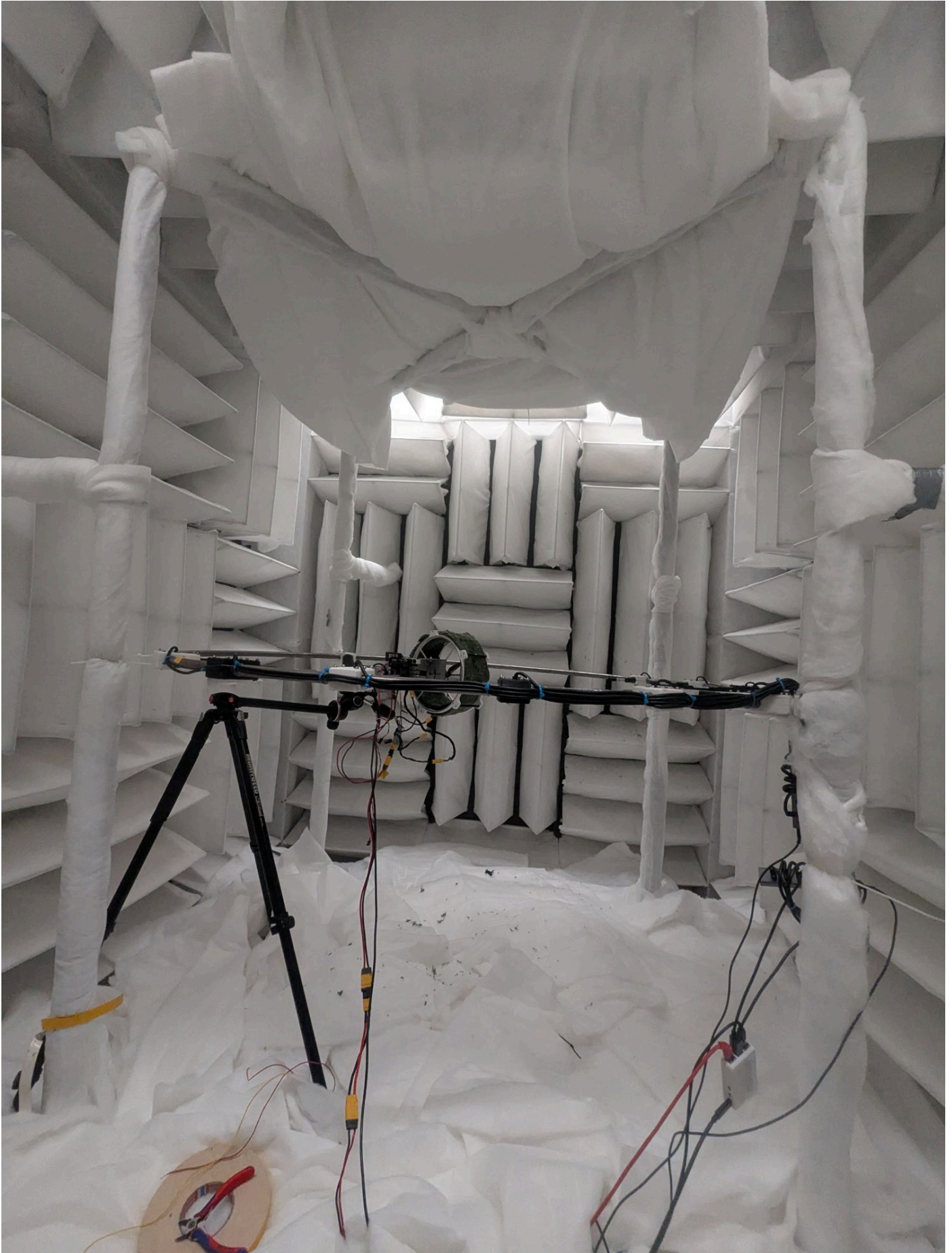
The chamber in the final configuration (carpet- reordered, photographed 5 Oct): the arc ring laid flat around the propeller rig at the hub, the speaker tripod on the left, batting on the floor and ceiling, wedges and lined pillars on the walls. The waterfall on the next page compares the start of day 3 with this state.
