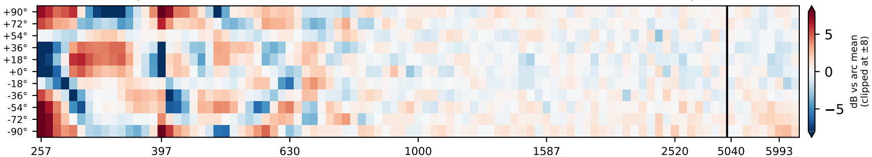
EVEN thick carpet (new levelled mount) — 2.540 dB below 3 kHz (2026-09-24/floor-even-carpet)
