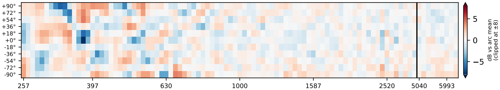
heaped carpet, no wedges (new levelled mount) — 1.443 dB below 3 kHz (2026-09-24/center-levelled)
