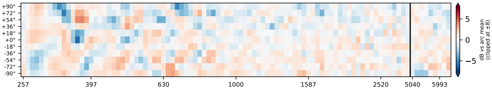
heaped carpet, no wedges (old tripod) — 1.324 dB below 3 kHz (2026-09-24/chaotic-carpet-3)
