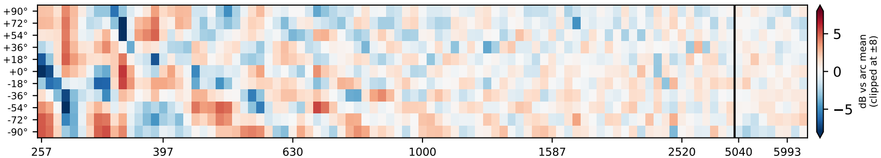
bare foam, everything removed (old tripod) — 2.054 dB below 3 kHz (2026-09-24/floor-no-wedges)
