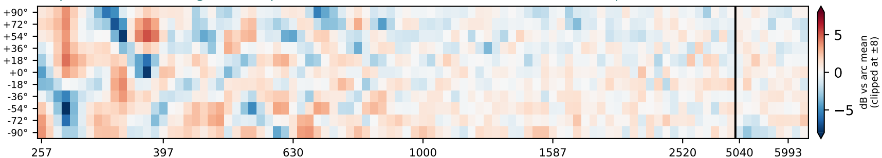
carpet laid flat, no wedges (old tripod) — 1.642 dB below 3 kHz (2026-09-24/carpet-added)
