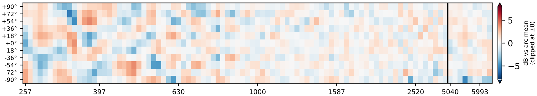
wedges only (old tripod) — 1.400 dB below 3 kHz (2026-09-24/bare-day2)
