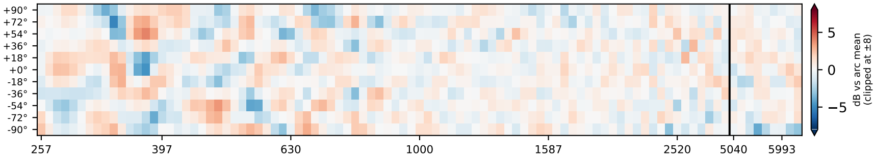
wedges + Thinsulate (old tripod) — 1.277 dB below 3 kHz (floor-carpet)
