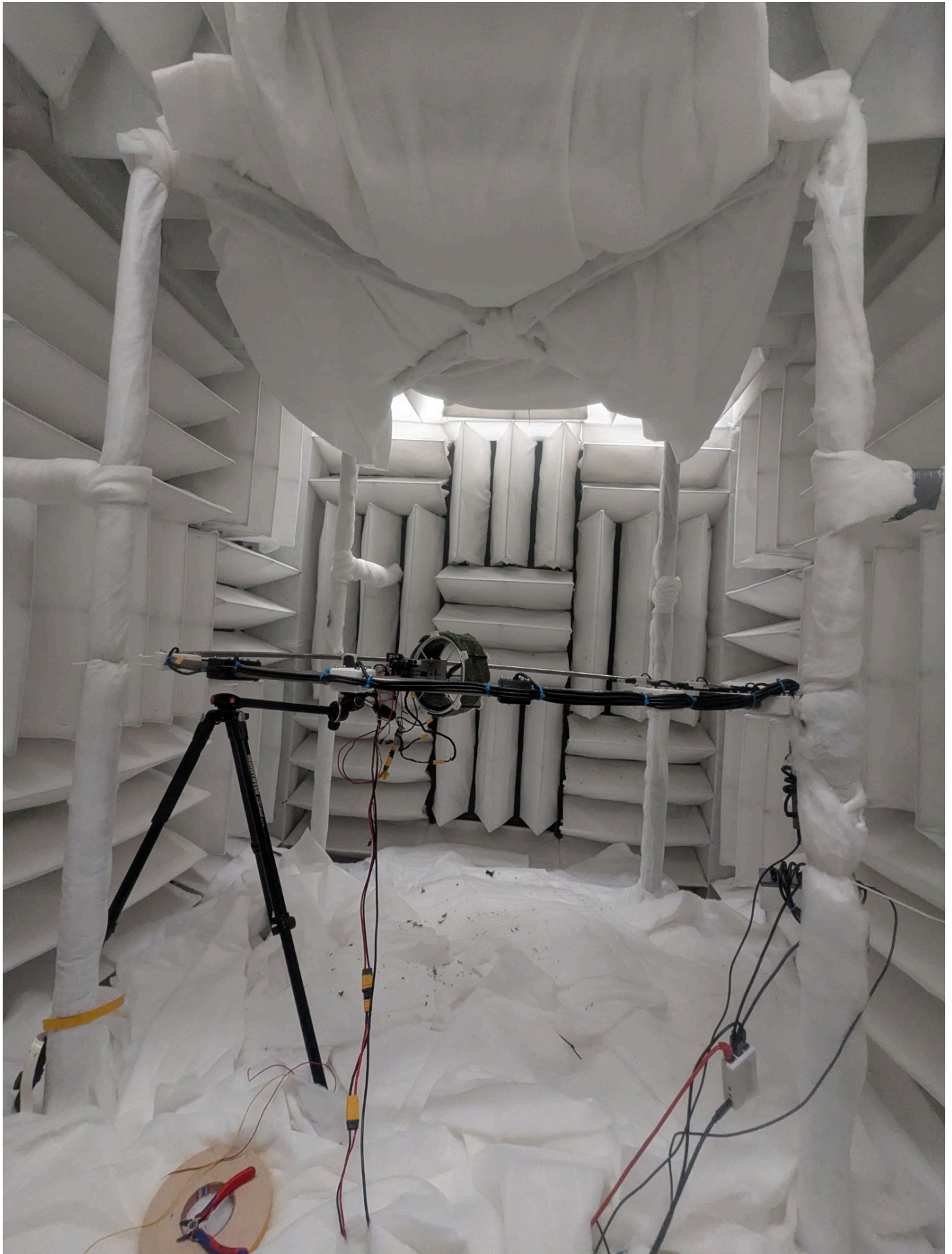
The chamber in the final configuration (carpet - reordered, photographed 5 Oct): the arc ring laid flat around the propeller rig at the hub, the speaker tripod on the left, batting on the floor and ceiling, wedges and lined pillars on the walls. The waterfall on the next page compares the start of day 3 with this state.
