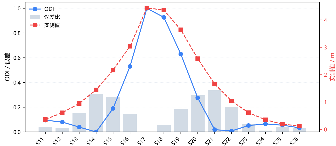
surface - 误差趋势 - 测线2
