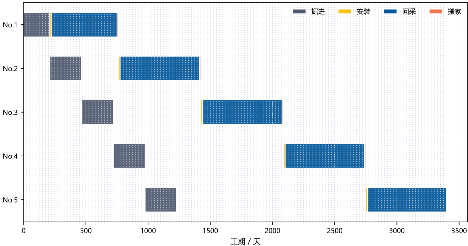
5-采掘接续.miningplan - Succession Gantt
