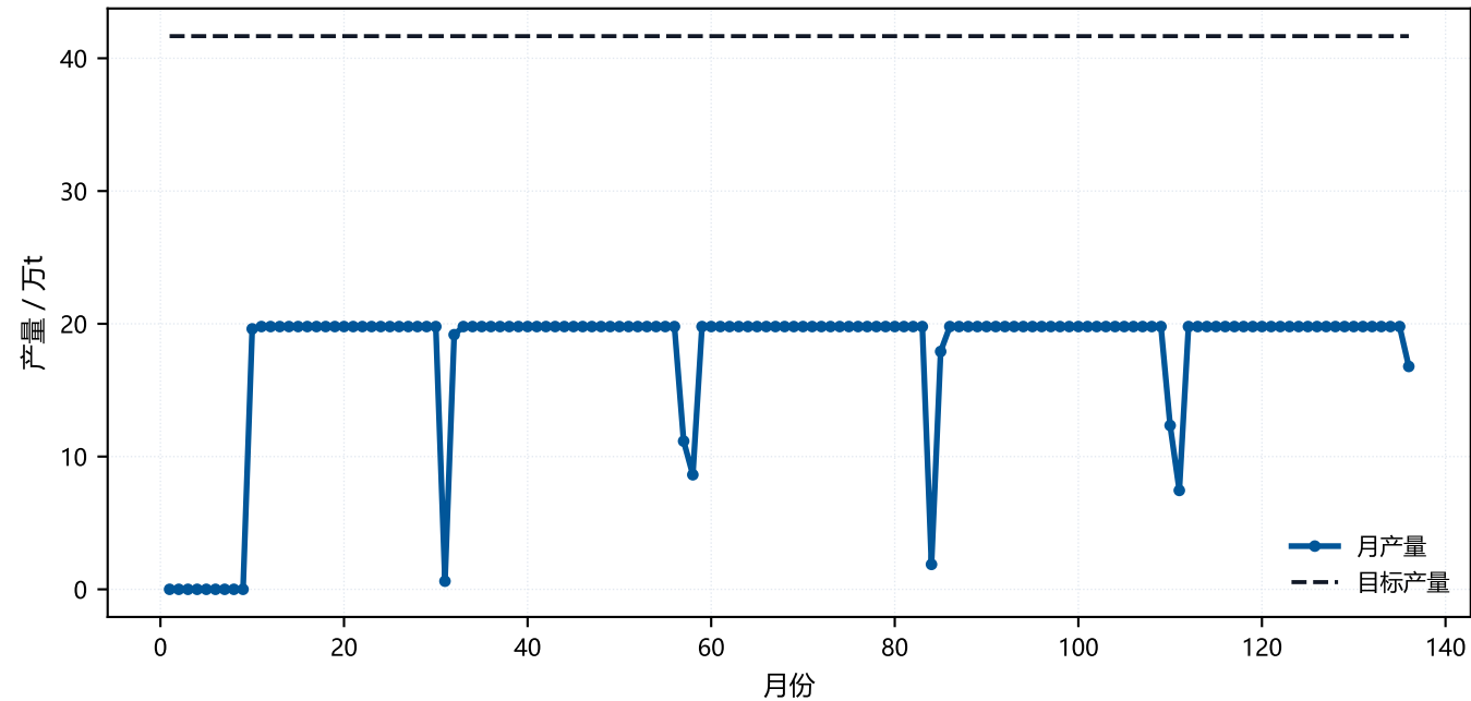
5-采掘接续.miningplan - Monthly Production
