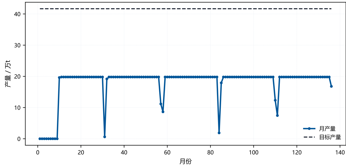
5-采掘接续.miningplan - Monthly Production
