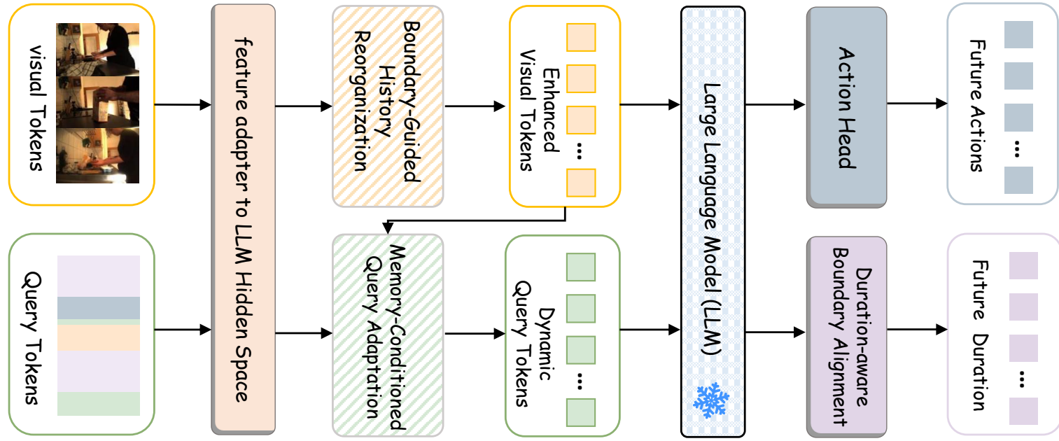
(a) ForeAct-LLM
