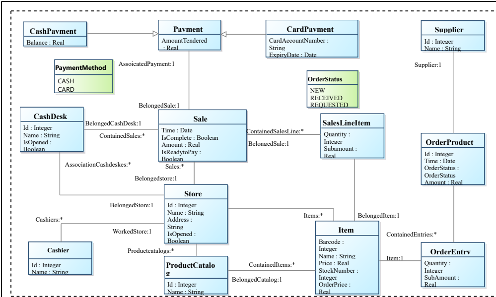
(a) Conceptual Class Diagram
