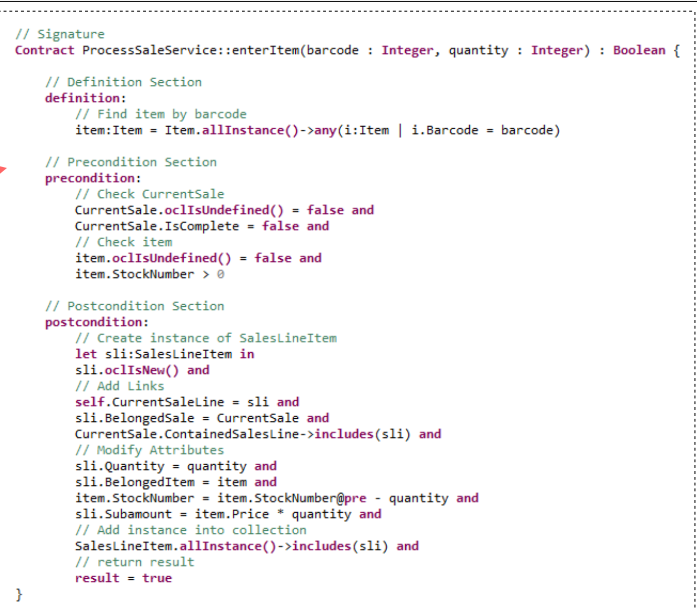
(d) Contract of System Operation "enterItem"
