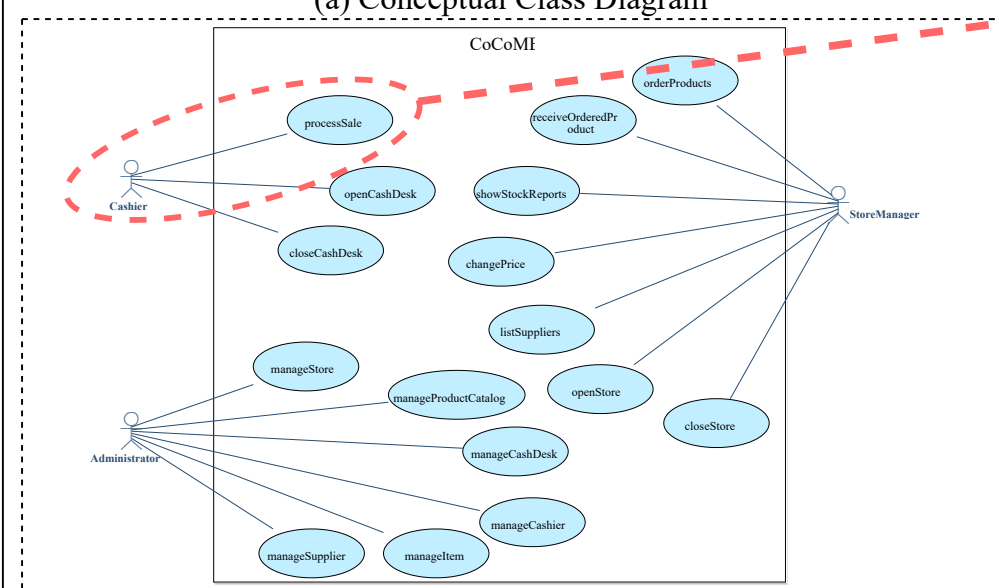
(b) Use Case Diagram
