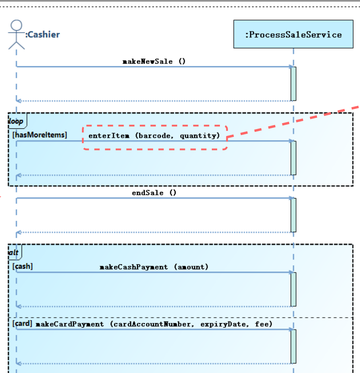
(c) System Sequence Diagram of Use Case "ProcessSale"
