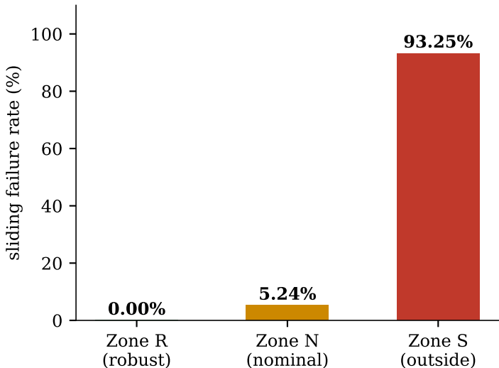
Mode verification (20,000 draws)
