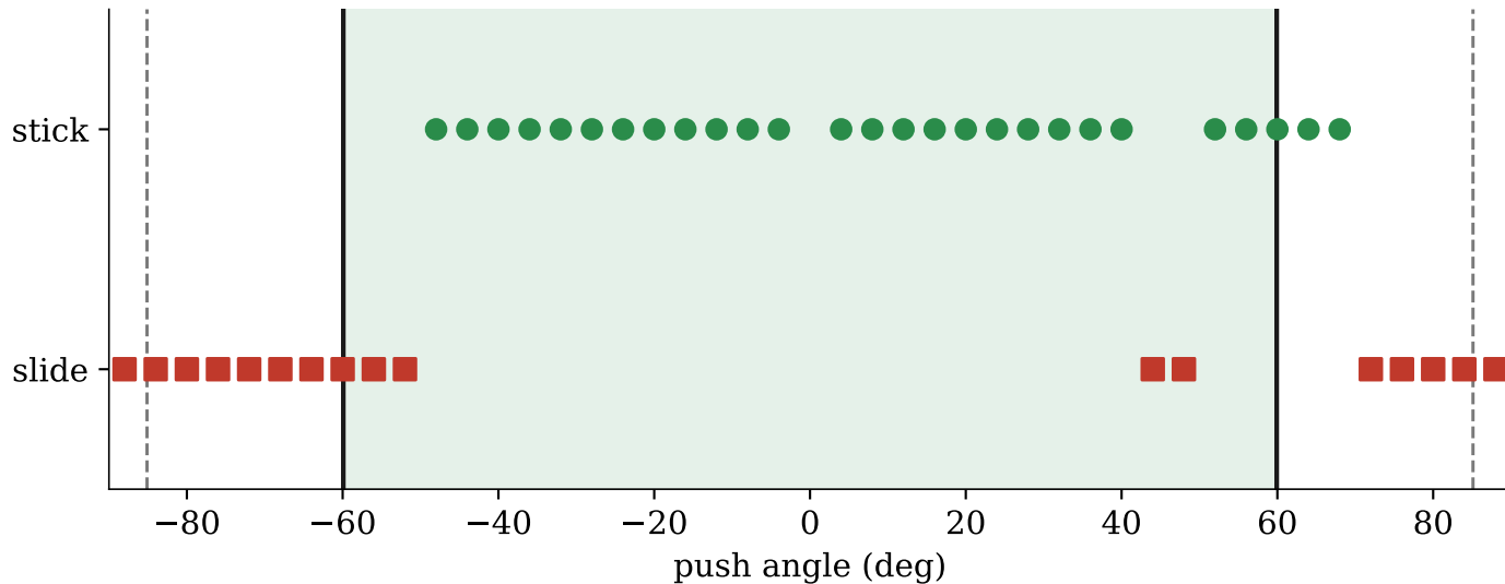
(a) Simscape Multibody stick/slide sweep (central realization \mu_0=0.45 , c_0=0.06 ; 84.1% accuracy, 37/44)
