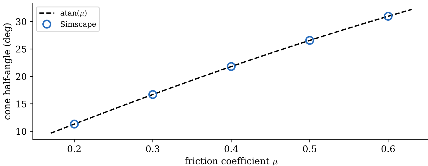
(b) Simscape \mu -sweep recovers \text{atan}(\mu) exactly (max err \leq 0.00^\circ )
