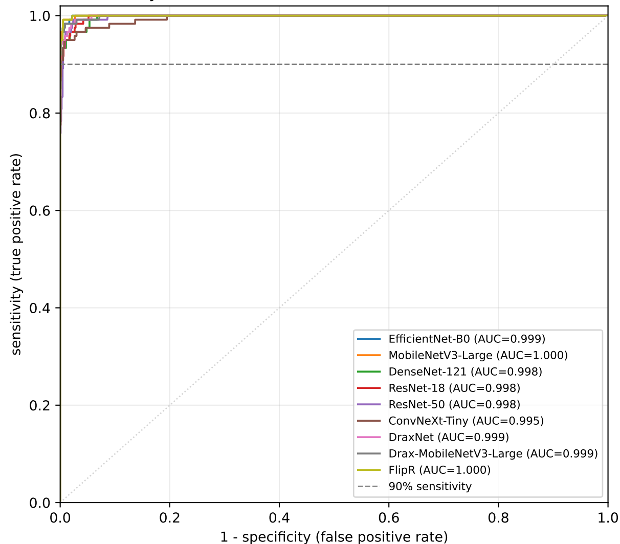
Binary TB discrimination ( P(tb) ) on the held-out test set
