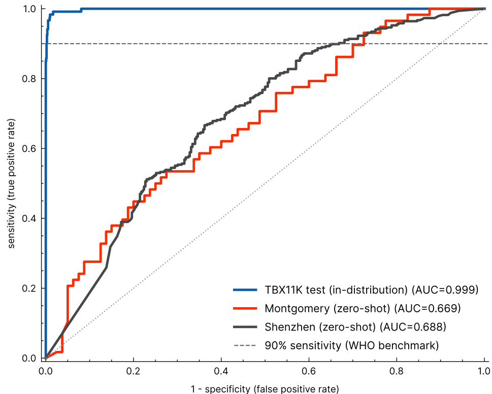
FlipR binary TB ROC: in-distribution vs unseen sites
