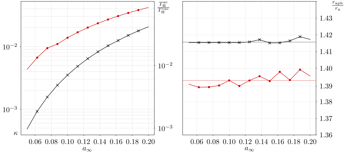
Figure 4: Dependence of the acoustic-horizon thermodynamics and lensing geometry on the asymptotic sound speed a_\infty , for \gamma = 5/3 (monatomic gas: red, filled circles) and \gamma = 4/3 (radiation-dominated plasma: black, crosses). (left) The surface gravity \kappa rises monotonically by more than an order of magnitude as a_\infty grows and the sonic point migrates inward toward the strong-field region; the right axis gives the analogue Hawking temperature relative to vacuum, 2\kappa = T_H^{\text{ac}}/T_H^{\text{vac}} . (right) The photon-sphere ratio r_{\text{aph}}/r_a stays nearly constant over the same range (dotted horizontal lines mark the means, \approx 1.39 for \gamma = 5/3 and \approx 1.42 for \gamma = 4/3 ), so the acoustic photon sphere tracks the horizon at a fixed multiple set mainly by the equation of state. Tabulated values at a_\infty = 0.05, 0.10, 0.15, 0.20 are listed in Table 4.
