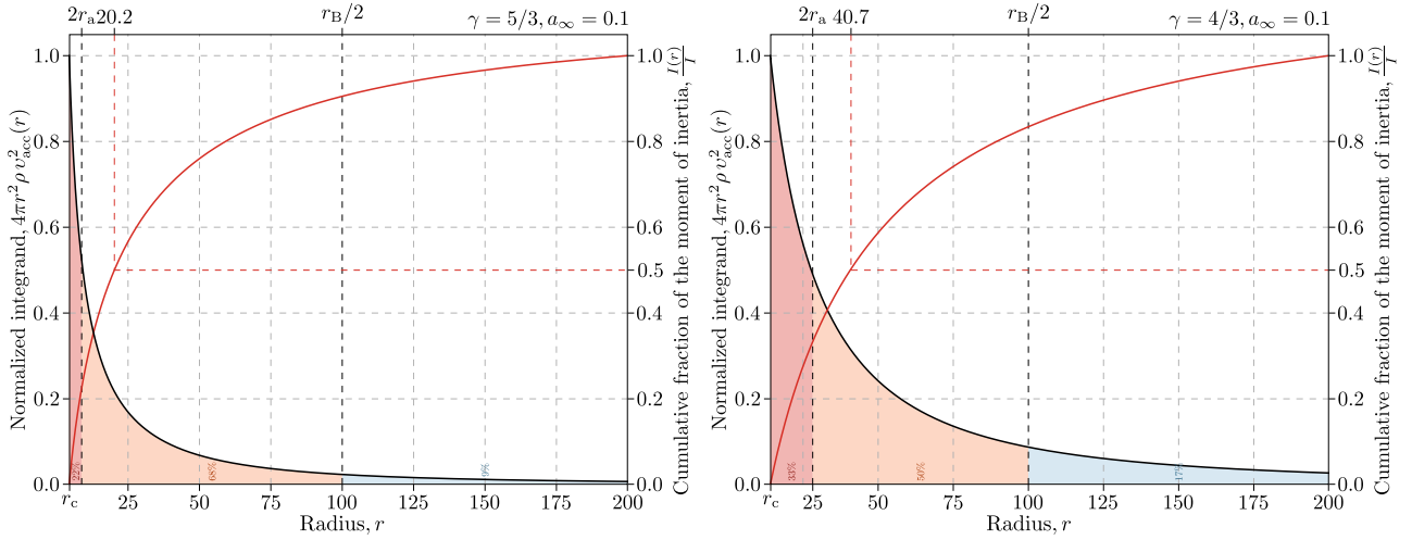
Figure 2: Integrant 4\pi r^2 \rho v_{\text{acc}}^2(r) of (19), normalized to its maximum value, as a function of r (in units of r_g ) for a_\infty = 0.1 . Left panel: \gamma = 5/3 ; right panel: \gamma = 4/3 . The shaded regions highlight the contributions of three radial intervals: [r_c, 2r_a] (acoustic-horizon region), [2r_a, r_B/2] (intermediate zone), and [r_B/2, r_B] (outer zone). The vertical dashed line marks r_c . The numerical fractions of the contribution of each interval to the total moment of inertia I are indicated in the insets.
