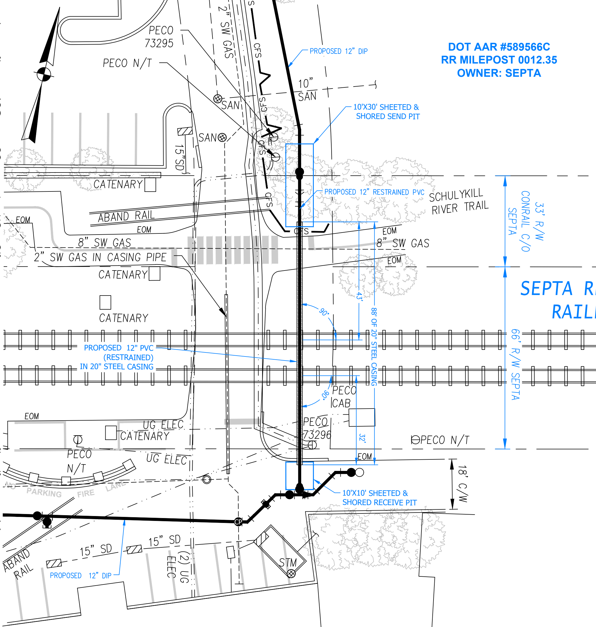
PLAN FOR SEPTA MANAYUNK/NORRISTOWN LINE SCALE - 1"=20'
