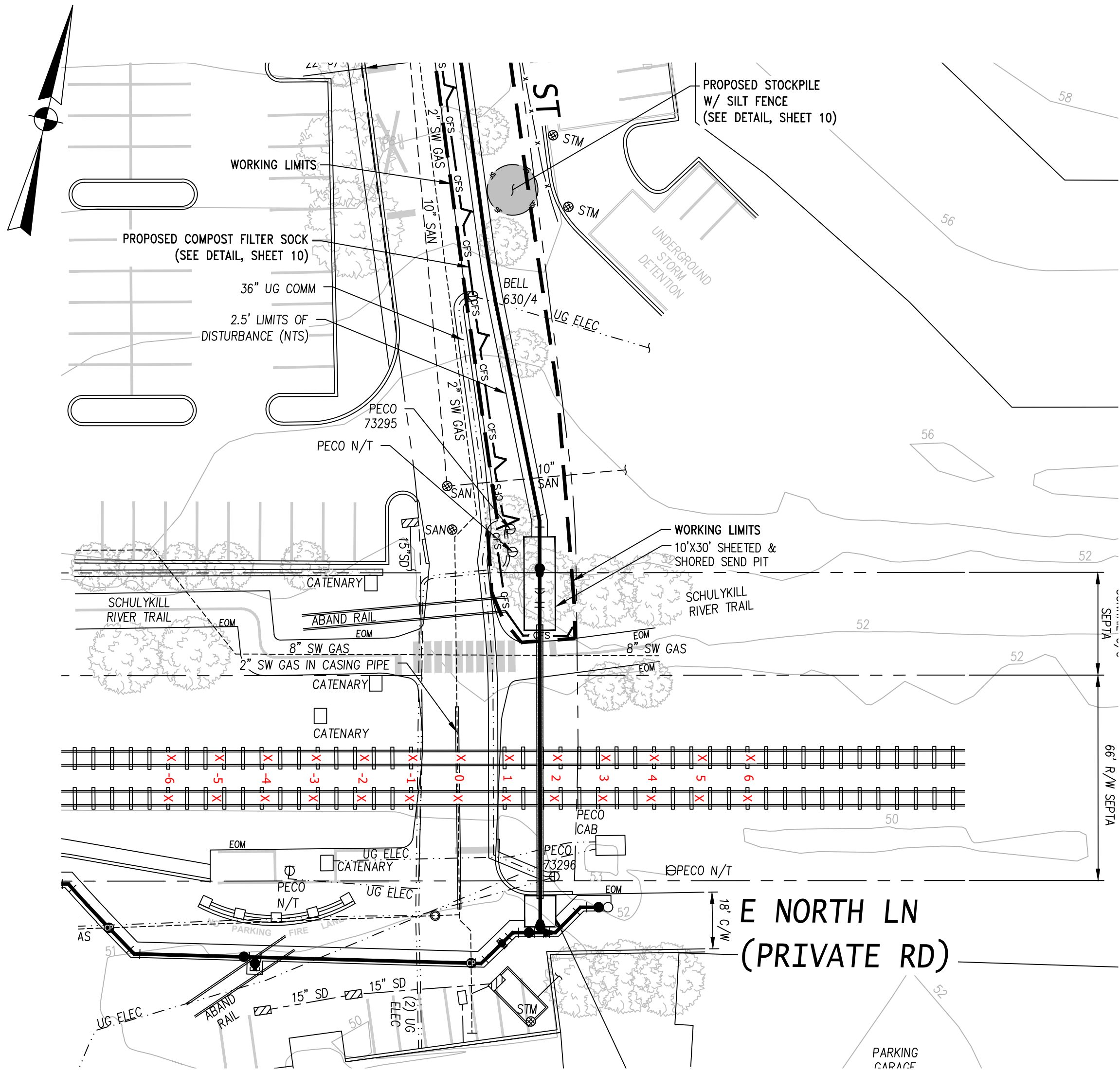
RAIL MONITORING PLAN SCALE - 1"=30'
