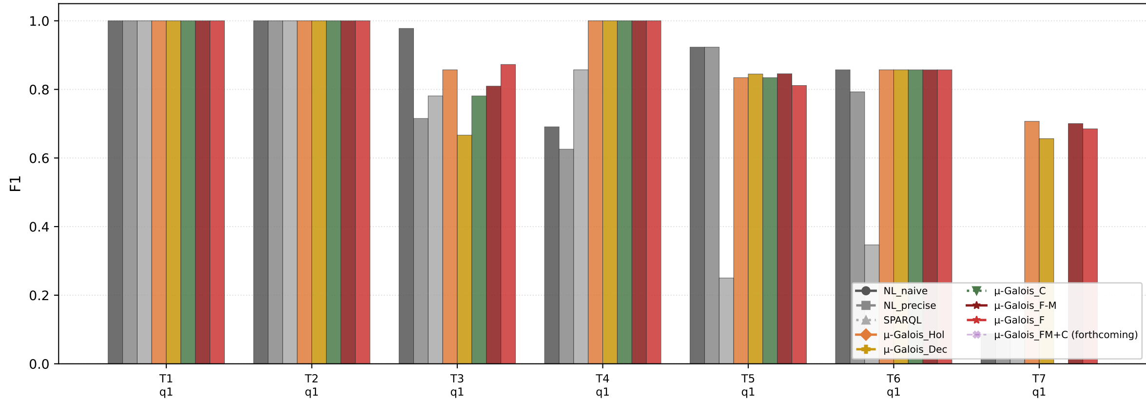
(Fig. RQ4-d) Per-query F1 — one representative query per template
