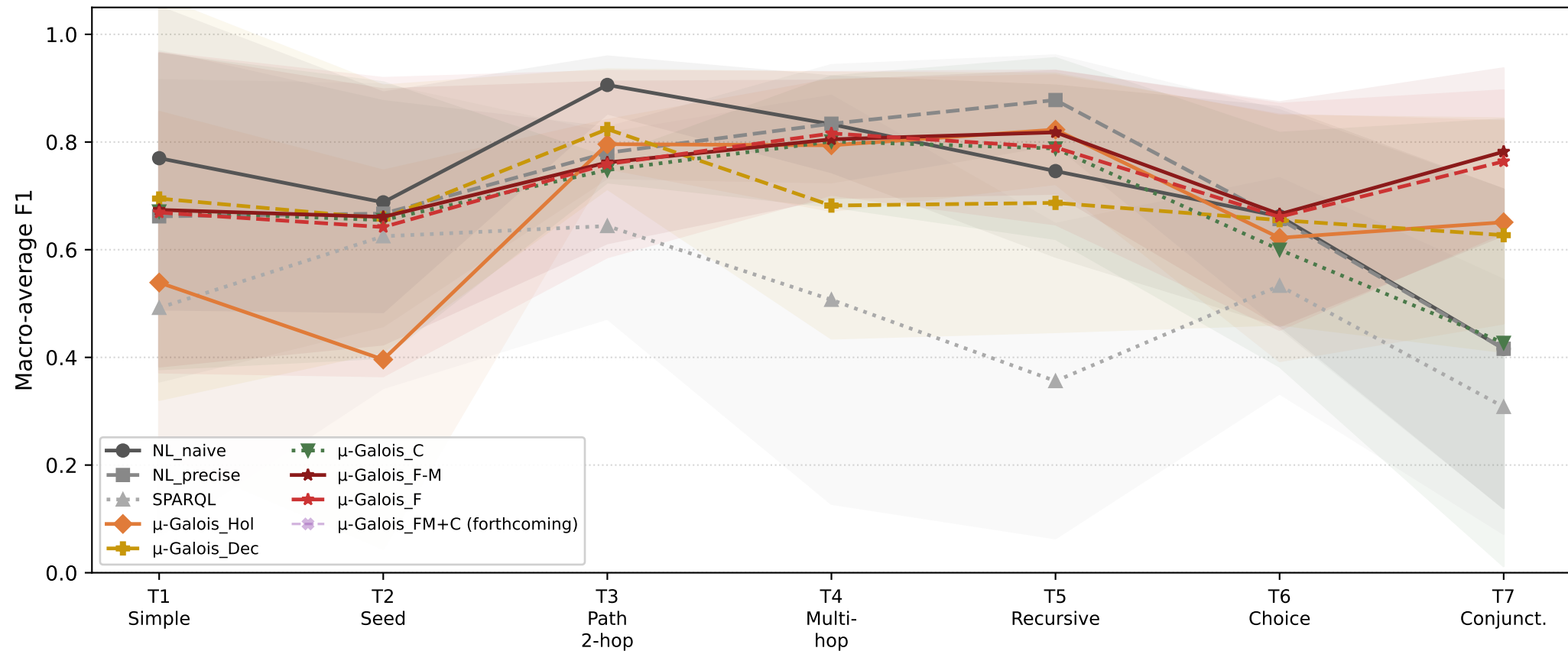
(Fig. RQ4-a) F1 per template — all models ordered by increasing query complexity →
