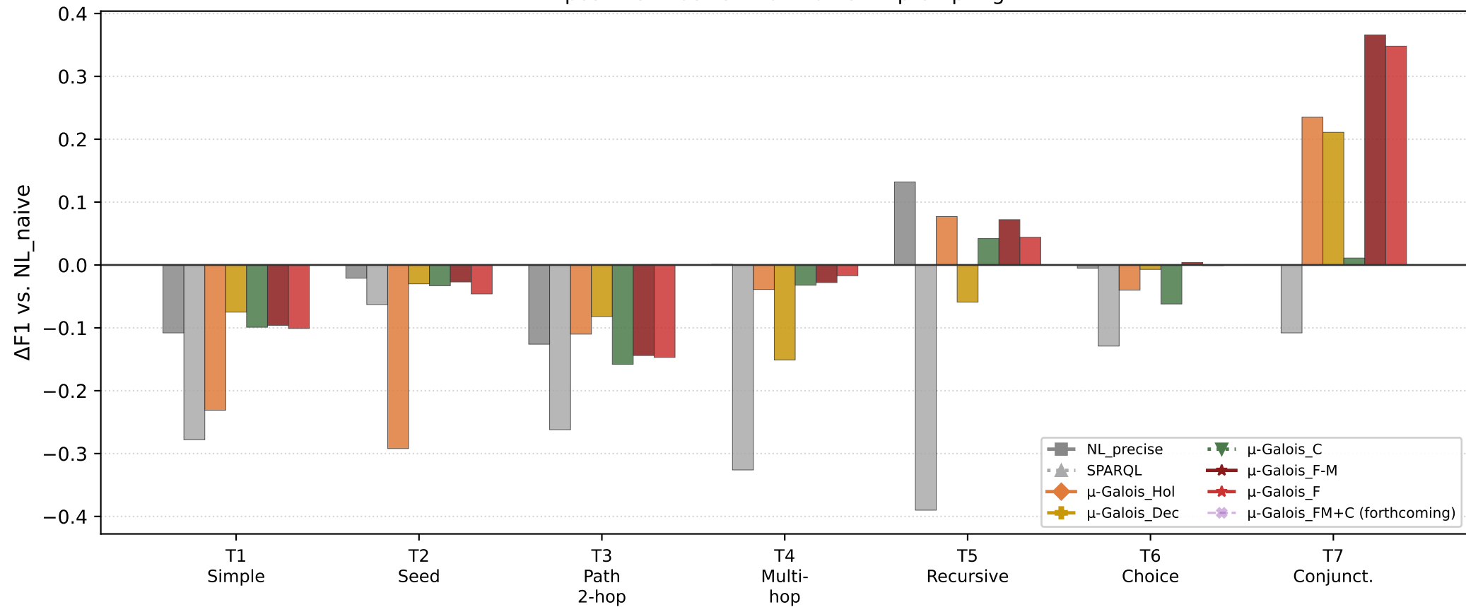
(Fig. RQ4-f) F1 gain over NL_naive baseline per template positive = better than naive NL prompting
